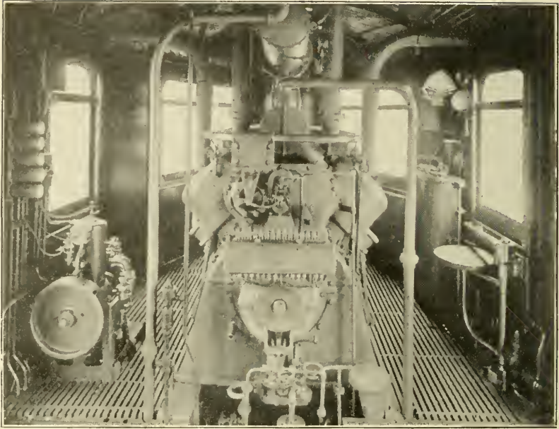
Fig. 13 Interior of Cab of General Electric Gas-Electric Car.
